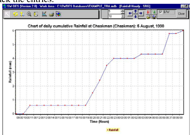
Figure 10: Plot of hourly rainfall simulated as observed by the analogous chart recorder
