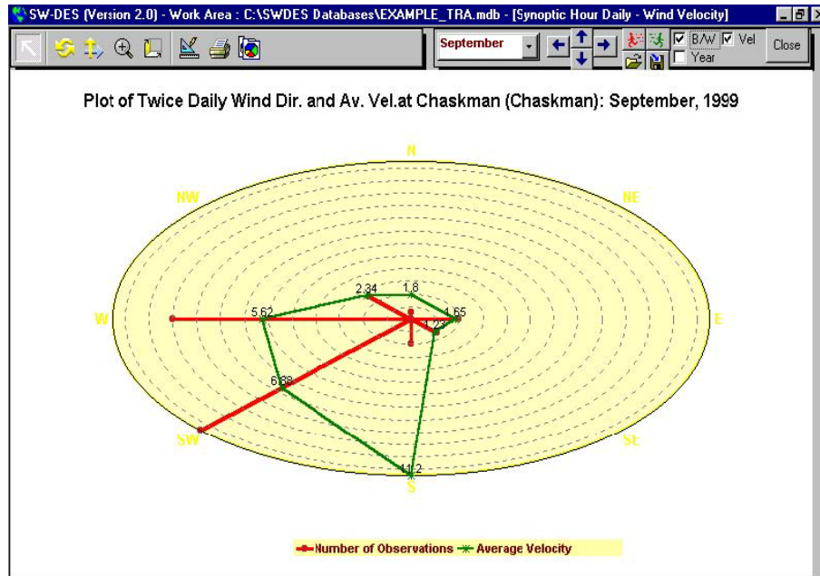
Figure 12: Plot of wind rose diagram
